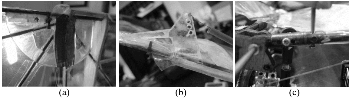
Figure 3. (a) Hinge; (b) Limiter; (c) Adapter
