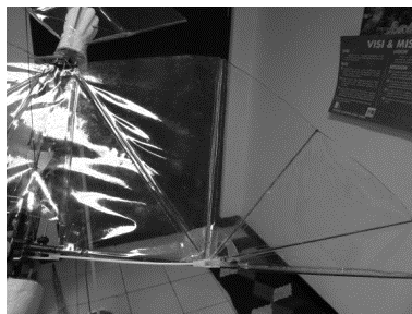
Figure 4. Wing mechanics
