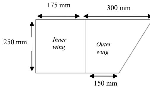
Figure 2. The dimensions of the ornithopter wing
